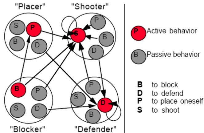
Figure 2.5: Influence Graph for the MICROB Soccer Robot Team [37]
